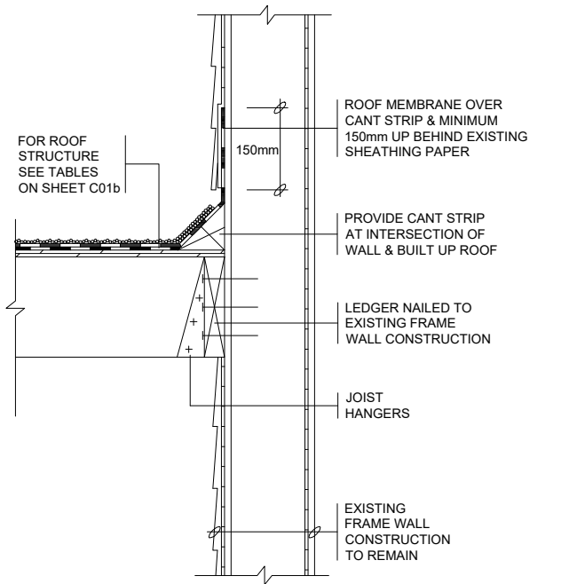
1 FRAME WALL
