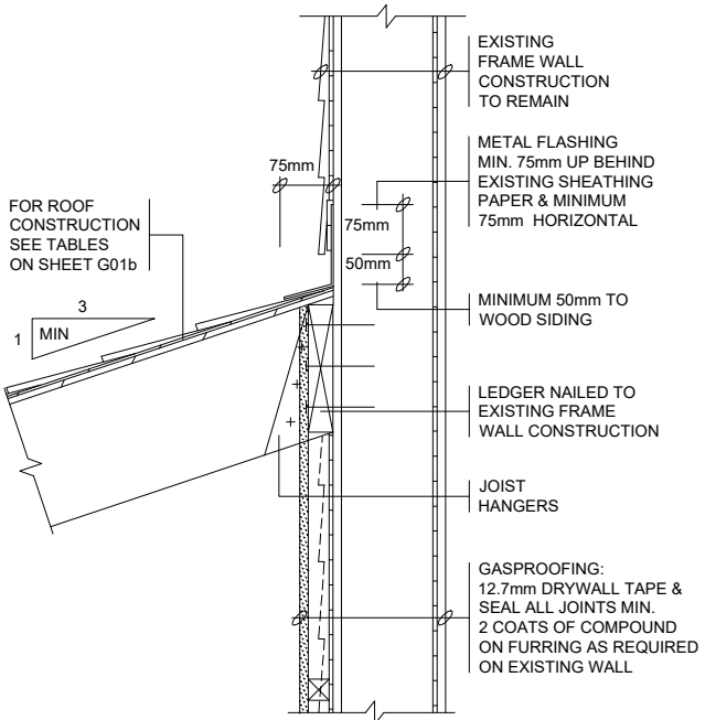
1 FRAME WALL
