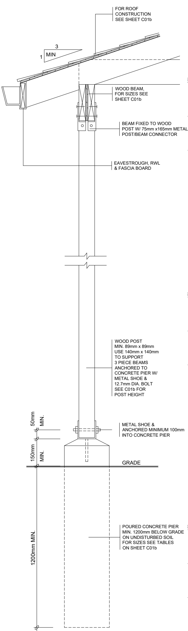
4 SUPPORT DETAIL
