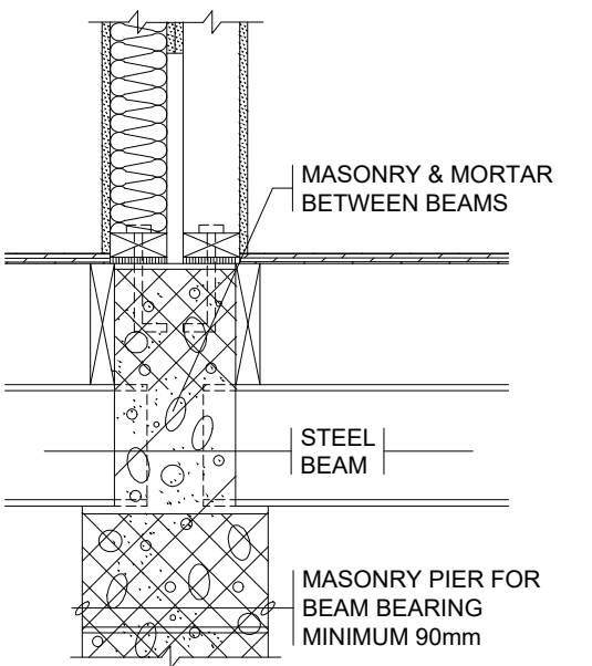
ALTERNATIVE 1
