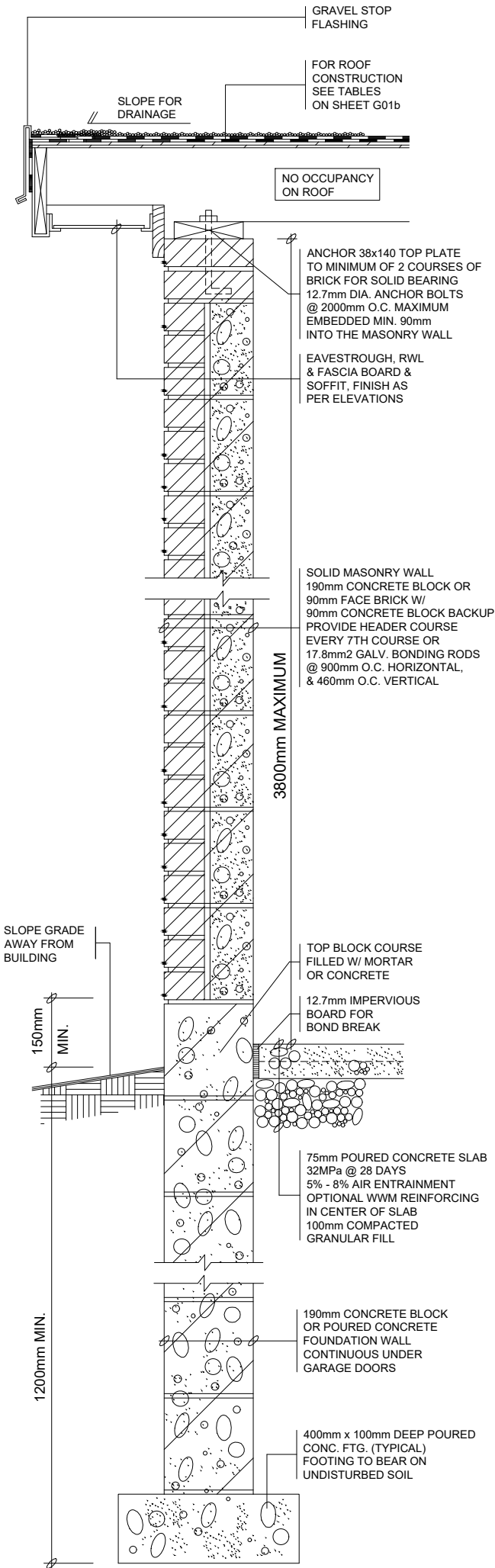
4 WALL SECTION
