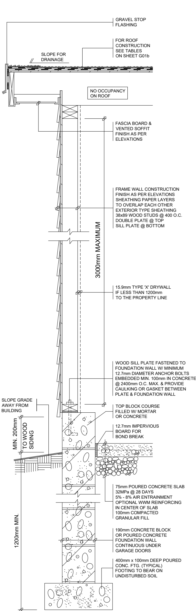
4 WALL SECTION
