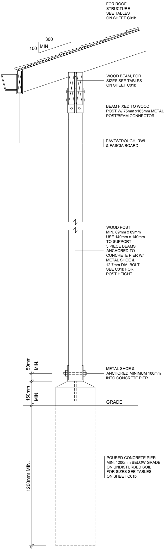
4 SUPPORT DETAIL
