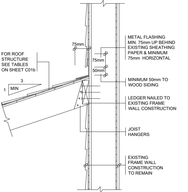
1 FRAME WALL
