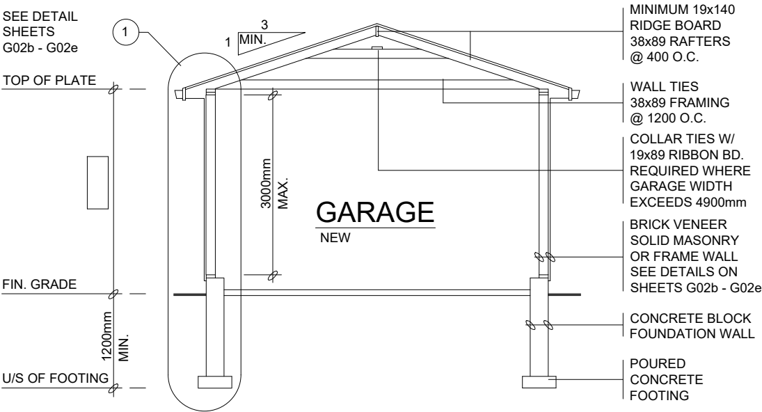
GABLE ROOF
