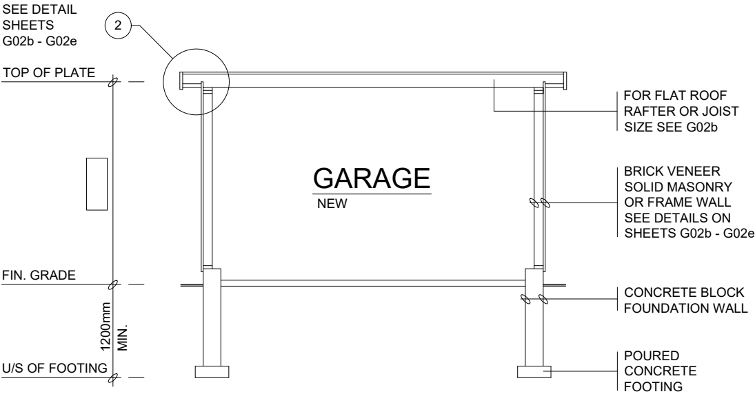
FLAT ROOF
