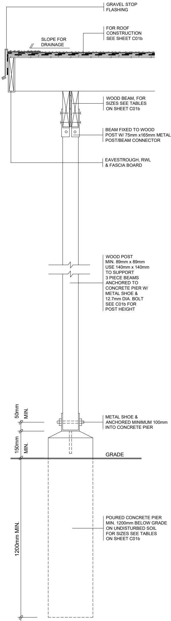
4 SUPPORT DETAIL
