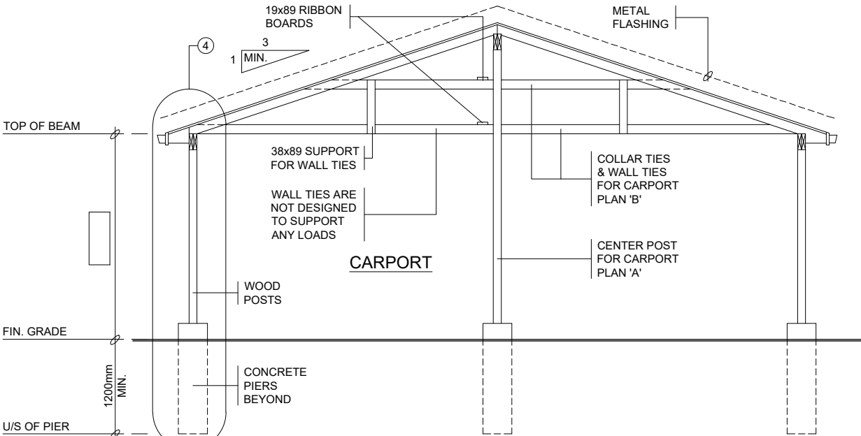
CARPORT SECTION
