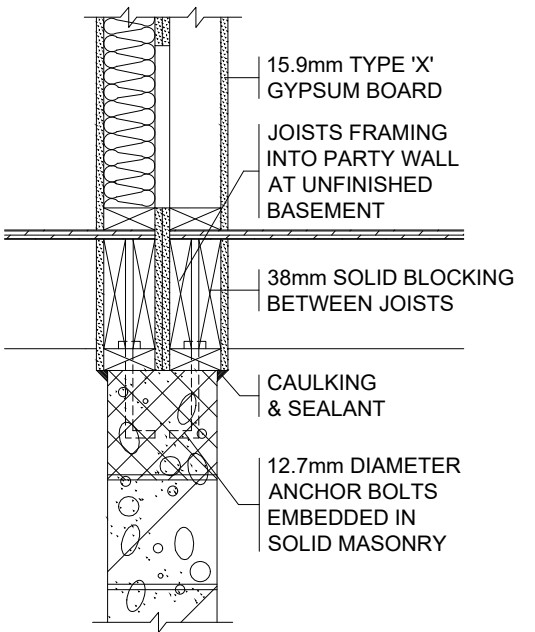
ALTERNATIVE 3
