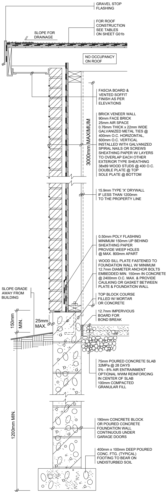
4 WALL SECTION
