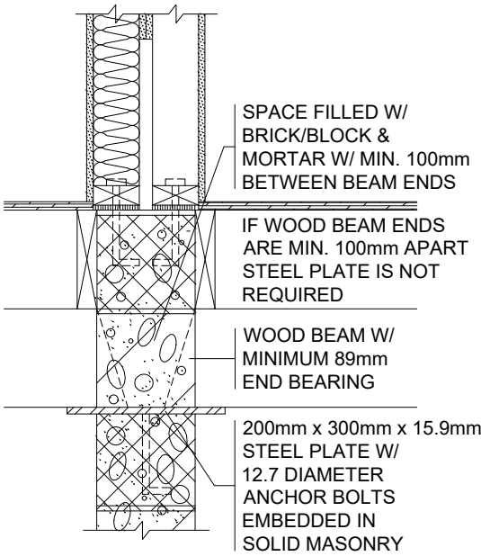
ALTERNATIVE 2
