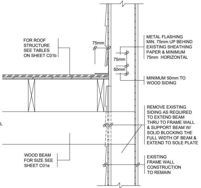
1 FRAME WALL
