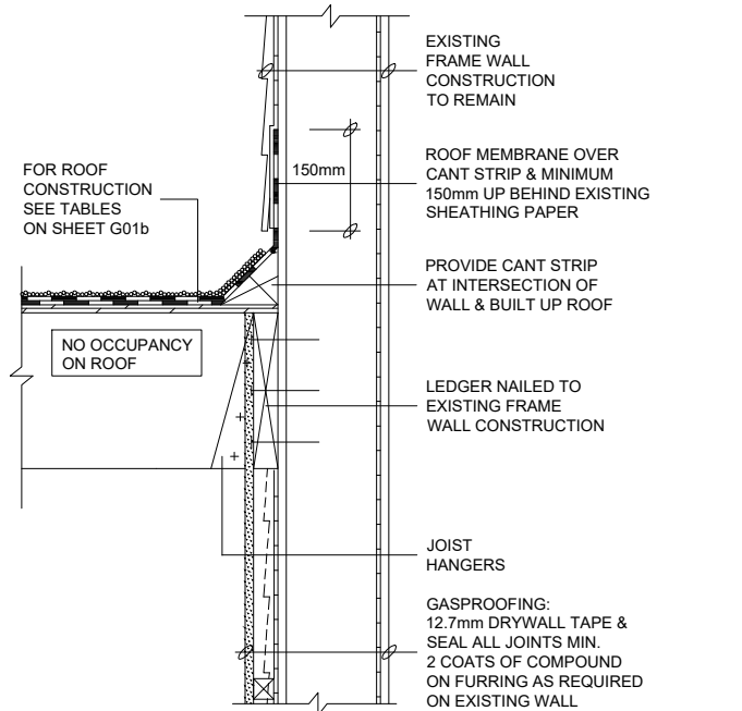
1 FRAME WALL
