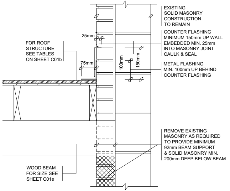
3 SOLID MASONRY WALL
