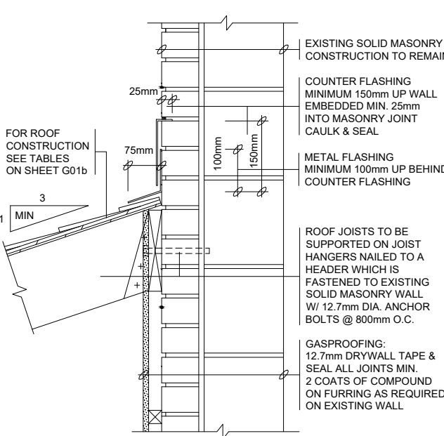
3 SOLID MASONRY WALL
