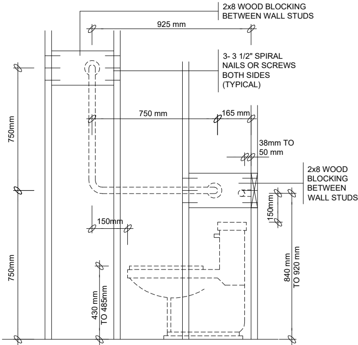
W.C. SIDE ELEVATION
