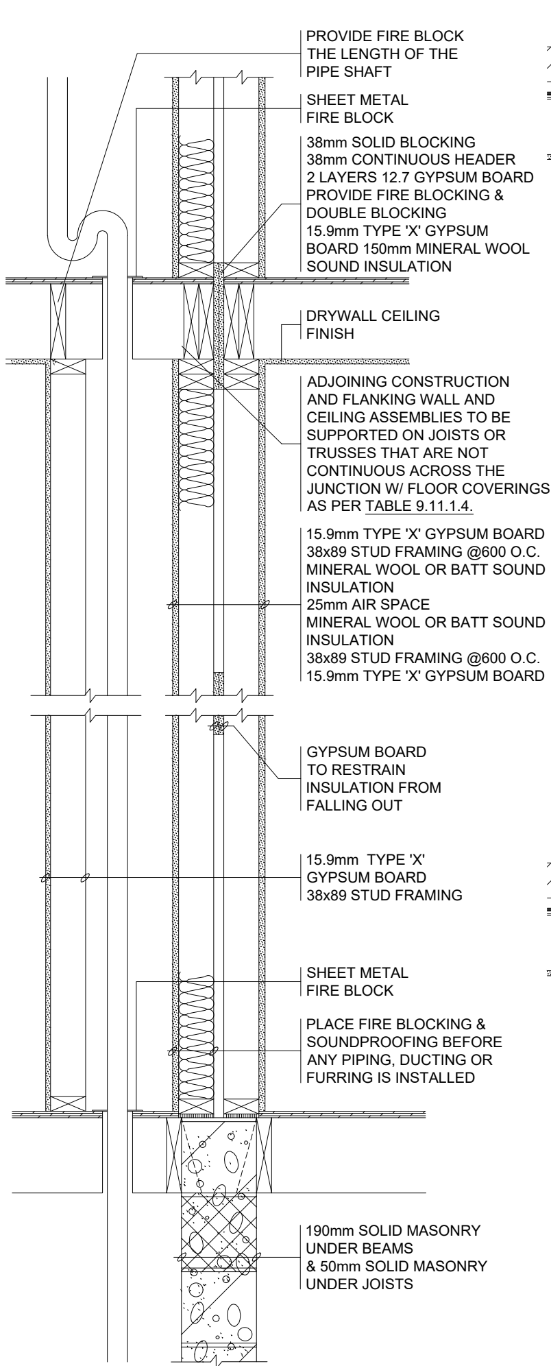
VERTICAL SECTION
